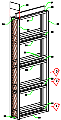
TIRROIR VERTICAL
